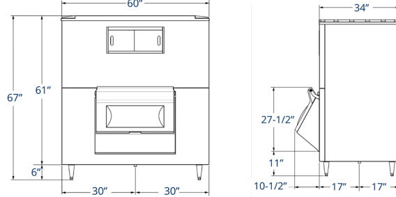
LB1760 - Front and Profile View
