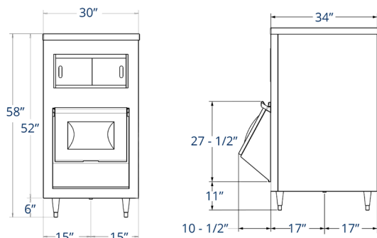
LB1460 - Front and Profile View
